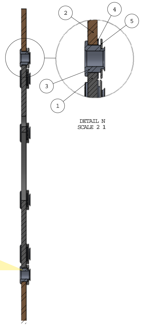
SECTION M-M
